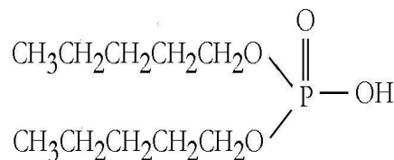
diamyl acid phosphate
