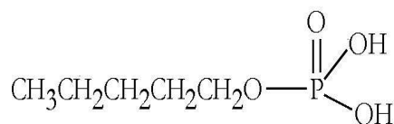
monoamyl acid phosphate
